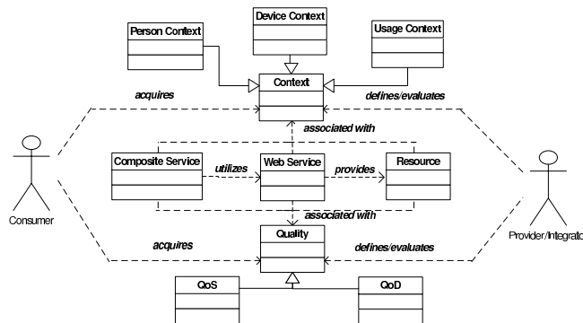
Fig. 3. Context and quality associated with composite services, Web services, and resources
