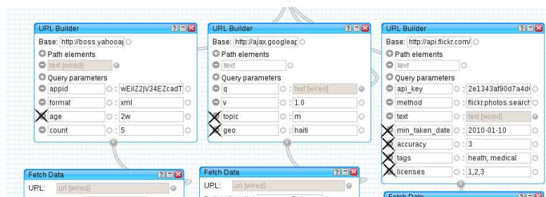
Fig. 2. Adding context and quality parameters (marked by X) during the service composition
